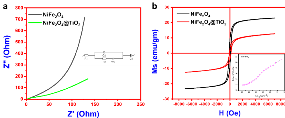
Fig 7: a) Impedance analysis (Nyquist plots) for pure NiFe 2 O 4 and NiFe 2 O 4 @TiO 2 b) M-H curves for pure NiFe 2 O 4 and NiFe 2 O 4 @TiO 2 (40% TiO 2 )
