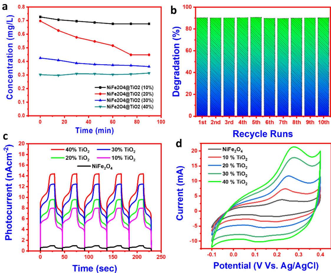
Fig 6: a) MO degradation Curve, b) recycling photocatalytic degradation of MO over NiFe 2 O 4 @TiO 2 (40%) composite, c) transient photocurrent densities profiles of photocatalysts, d) cyclic voltammograms of photocatalysts
